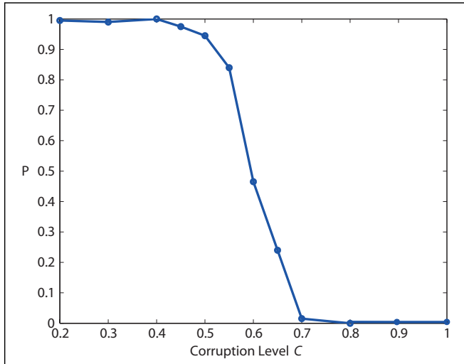
Figure 12 | Basin of attraction : Recognition probability P , as a function of input corruption C , measured with the protocol of Figure 11 . For corruption levels C > 0.65 , P falls below 25%, which implies that recognition fails in more than 75% of the trials.
